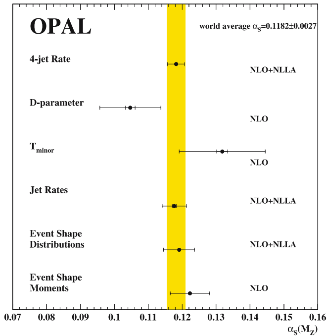
Fig. 6. The results of the fit to the four-jet rate, the D -parameter and T_{\text{min}} . The value of the strong coupling \alpha_S obtained from the four-jet rate represents our main result. The analyses of the D -parameter and T_{\text{min}} return larger uncertainties as discussed in Sect. 5.2. Results published by the OPAL collaboration using different predictions and event shapes are shown as well. The value of \alpha_S indicated by Jet Rates is obtained by [12]. The results of [13] are indicated as “Event Shape Distributions” and “Event Shape Moments”. The type of QCD prediction is indicated in the plot. The \alpha_S world average is taken from [37]
