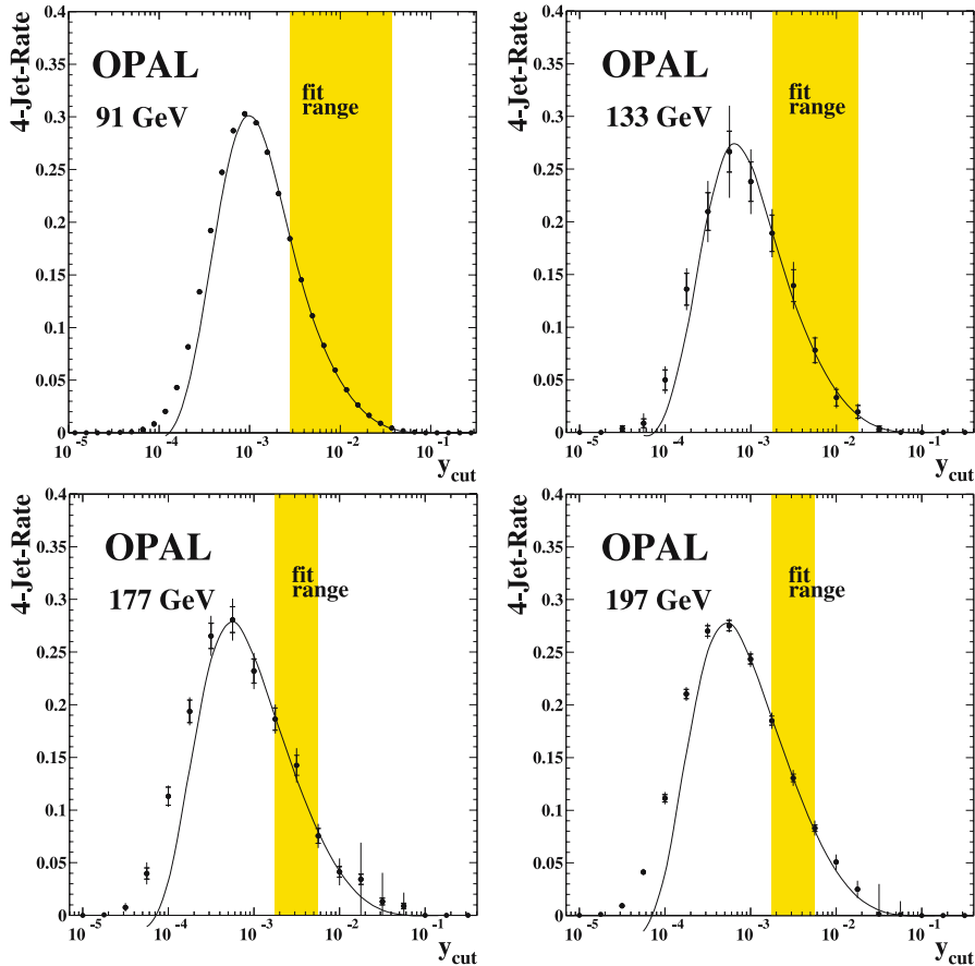
Fig. 2. The hadron-level four-jet rate distributions for energies between 91 GeV and 209 GeV. The error bars show the statistical (inner error bars) and experimental uncertainties added in quadrature. When not shown, the errors are smaller than the point size. The curves show the theory prediction after \chi^2 minimization within the fit range indicated. The fit range is determined as discussed in Sect. 5.1.1. The data points are strongly correlated and an enlarged fit range would lead to only a minor gain in statistical precision
