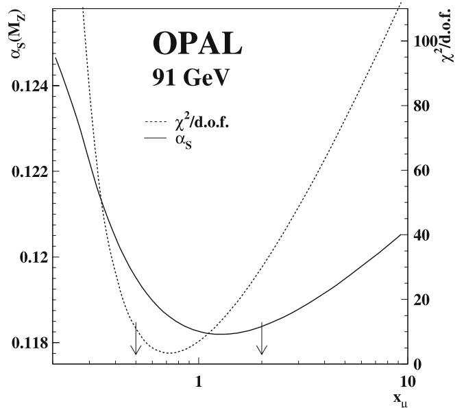
Fig. 4. The values of \alpha_S and \chi^2/\text{d.o.f.} from the fit to the four-jet rate at 91 GeV data as a function of the scale parameter x_\mu . The arrows indicate the variation 0.5 < x_\mu < 2.0 used to determine the theoretical systematic uncertainty
