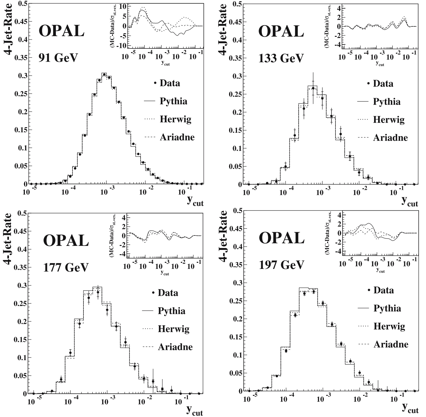
Fig. 1. The four-jet rate distribution at hadron level as a function of the y_{cut} resolution parameter obtained with the Durham algorithm. The four-jet rates are shown for the data corrected to the hadron level at four average centre-of-mass energies between 91 and 209 GeV together with predictions based on PYTHIA, HERWIG and ARIADNE Monte Carlo events generated at the averaged energy. The error bars show the statistical (inner error bars) and experimental uncertainties added in quadrature. Error bars not shown are smaller than the point size. The panel in each upper right corner shows the differences between data and Monte Carlo predictions, divided by the sum of the statistical and experimental error. For data points with no data events, the difference is set to zero
