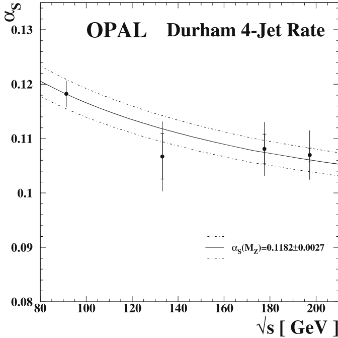
Fig. 3. The values for \alpha_S obtained by a fit to the four-jet rate with x_\mu set to 1.0 in the four energy intervals. The error bars show the statistical (inner error bars) and the total error. The statistical error at 91 GeV is smaller than the point size. The lines indicate the current world average from [37] with the one standard deviation uncertainty
