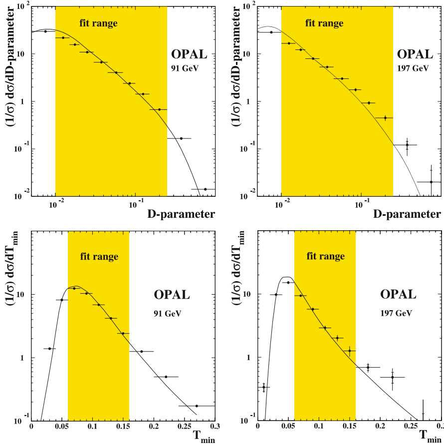
Fig. 5. The hadron-level D -parameter and T_{\min} distributions for energies of 91 GeV and 197 GeV. The error bars show the statistical (inner error bars) and experimental uncertainties added in quadrature. When not shown, the errors are smaller than the point size. The curves indicate the theory prediction after \chi^2 -minimization with the renormalization scale set to 1.0. The fit range is determined as discussed in Sect. 5.2
